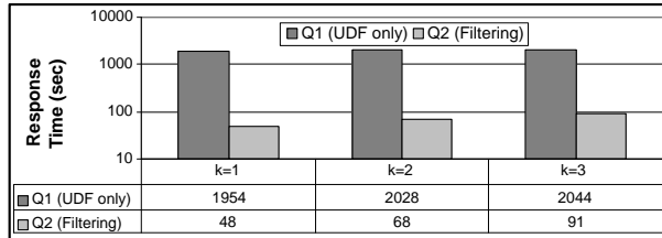
Figure 3: Executing Queries Q1 and Q2 over the Sample Database.
